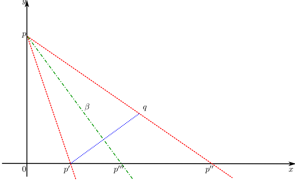
Figure 7: This is a schematic representation of the configuration if \tau \geq \theta . The proof for case \tau \leq \theta is identical.
