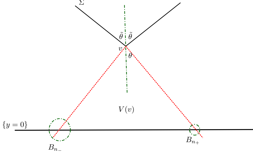
Figure 6: If v talks to points in two distinct balls, \mathcal{L}^1(V(v) \cap \{y = 0\}) is “large”, thus the turning angle \operatorname{TA}(v) is “large”. But there is not enough mass to allow for such large turning angle. Here we omitted representing the balls (if these exist) B_n with n_- < n < n_+ . The relation between \theta and \tilde{\theta} is 2\theta = \pi - 2\tilde{\theta} = \pi - \operatorname{TA}(v) .
