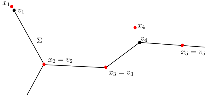
Figure 1: Some examples of vertices ( \{v_1, \dots, v_5\} in figure). The red dots denote the support ( \{x_1, \dots, x_5\} in figure) of the reference measure. Here d(x_i, \Sigma) = |x_i - v_i| , i = 1, \dots, 5 .
